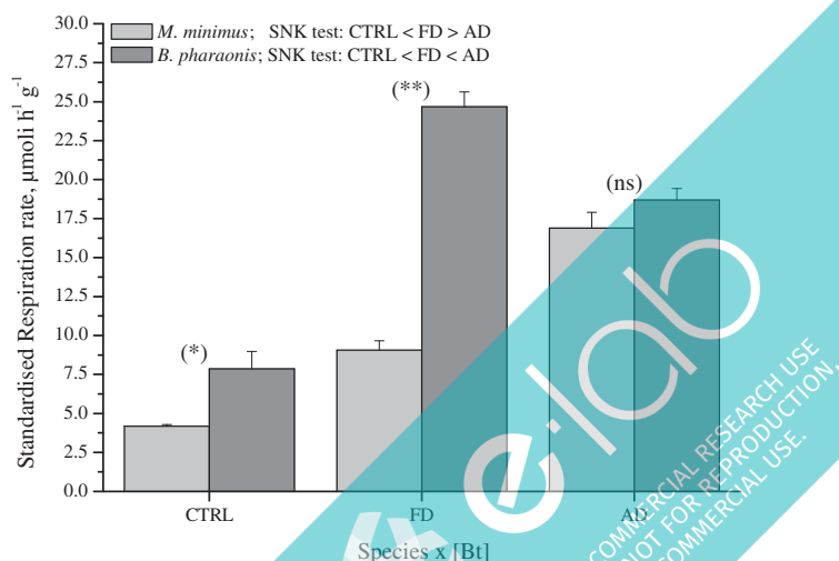
Fig. 2. Respiration rates of both species at varying Bt concentrations; FD = 45 \mu\text{L L}^{-1} , AD = 90 \mu\text{L L}^{-1} , CTRL = control.
