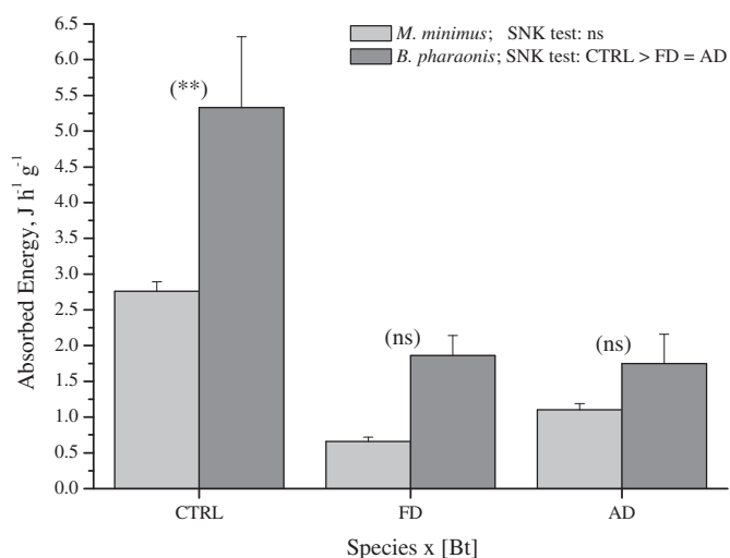
Fig. 4. Absorbed energy rates of both species at varying Bt concentrations; FD = 45 \mu\text{L L}^{-1} , AD = 90 \mu\text{L L}^{-1} , CTRL = control.
