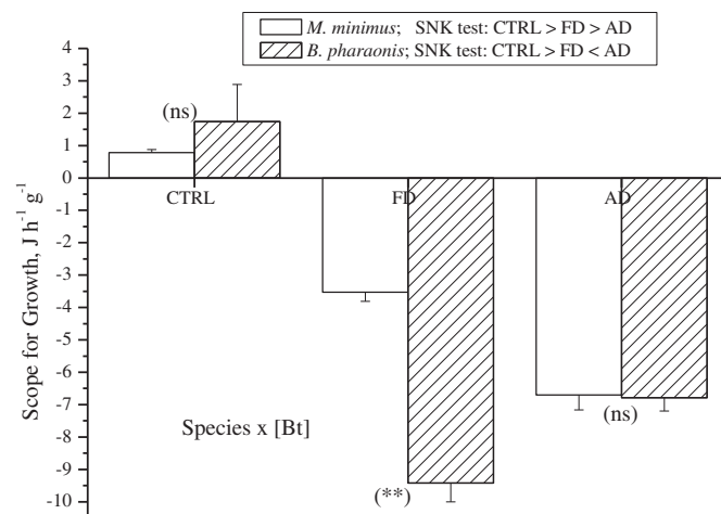
Fig. 5. Scope for Growth of both species at varying Bt concentrations; FD = 45 \mu\text{L L}^{-1} , AD = 90 \mu\text{L L}^{-1} , CTRL = control.
