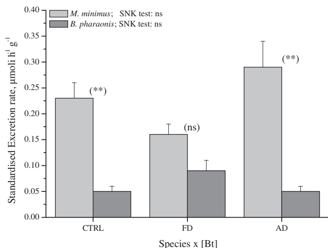
Fig. 3. Excretion rates of both species at varying Bt concentrations; FD = 45 \mu\text{L L}^{-1} , AD = 90 \mu\text{L L}^{-1} , CTRL = control.
