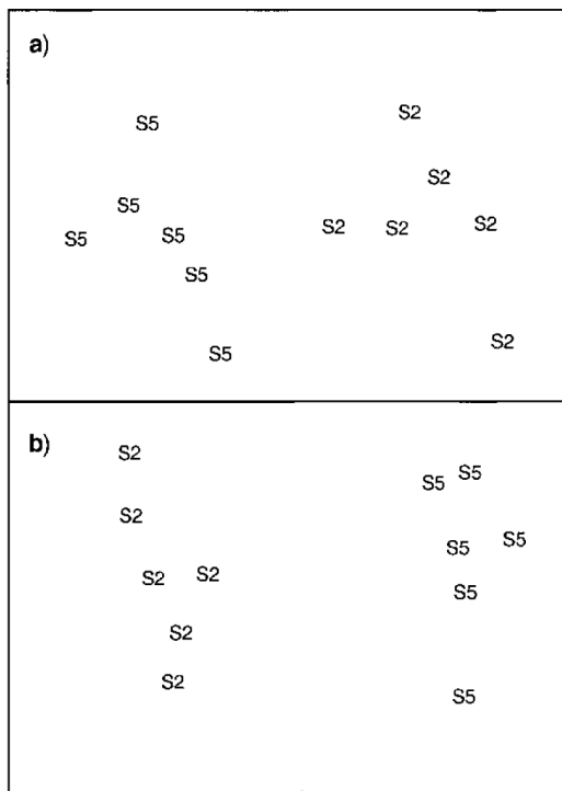
FIGURE 6 Non-metric multidimensional scaling ordinations (n-MDS) of (a) d N and (b) d C values of organic matter sources and consumers based on the normalized Euclidean distance similarity matrix. S5: Sector 5; S2: Sector 2.
