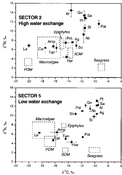
FIGURE 5 \delta^{13}\text{C} vs. \delta^{15}\text{N} (+S.D.; ‰) for organic matter sources (dashed squares) and consumers from the two sampling sectors. For acronyms, see Table III.
